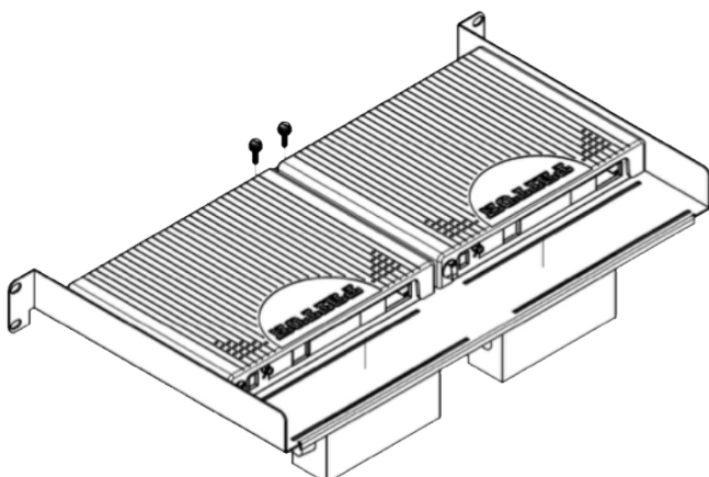
Figure 2 - Products with connectors facing rear
