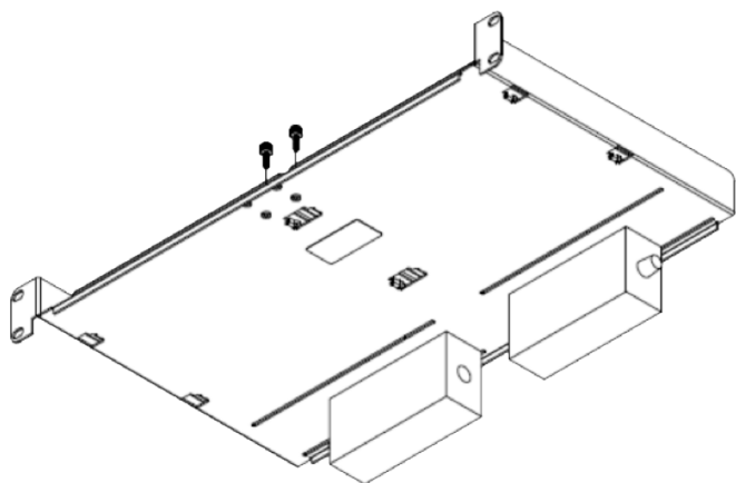
Figure 3 - Power Supplies mounted underneath
